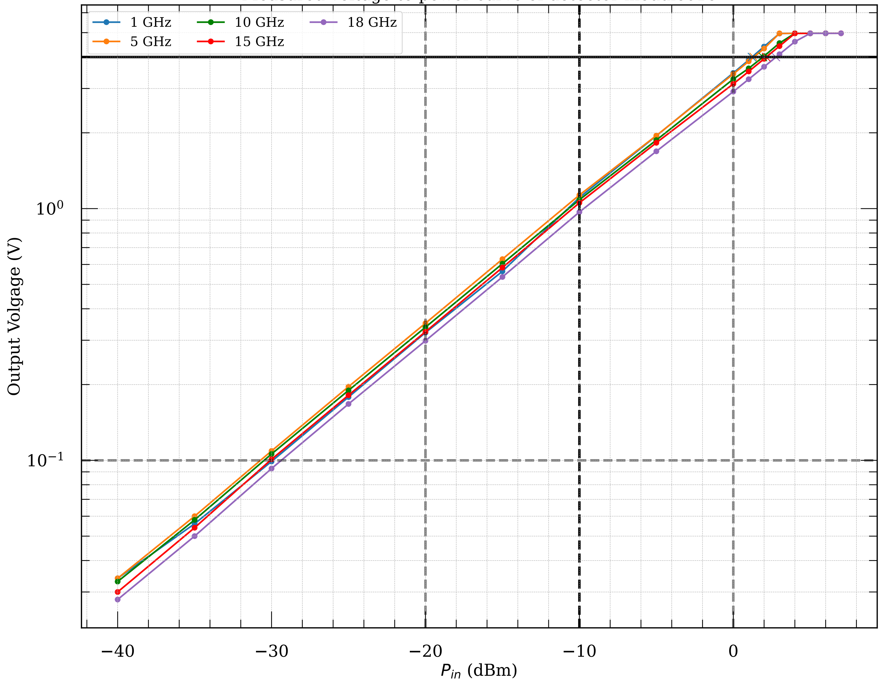
Measured voltage-to-power curve of detector module016
